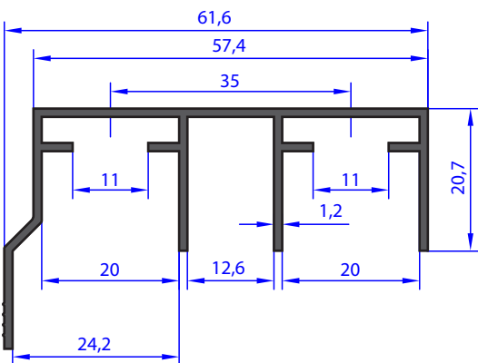
AB 95505 WEIGHT 0.552 Kg/m
