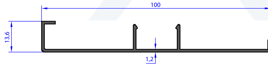
AB 95305 WEIGHT 0.468 Kg/m
