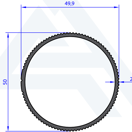
AB 97176 WEIGHT 0.714 Kg/m
