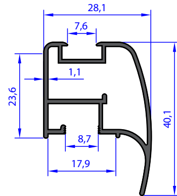
A.3202 WEIGHT 0.398 Kg/m
