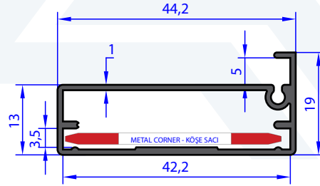
AB 96837 WEIGHT 0.379 Kg/m
