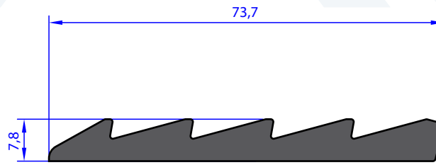
AB 95049 WEIGHT 1.183 Kg/m
