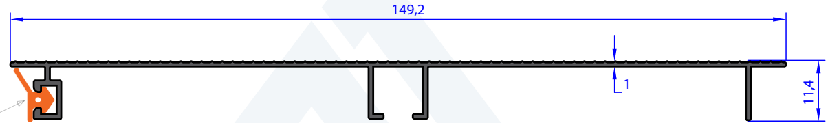
BFTL - 3840 BAZA FİTİLİ - (BASE GASKET)
