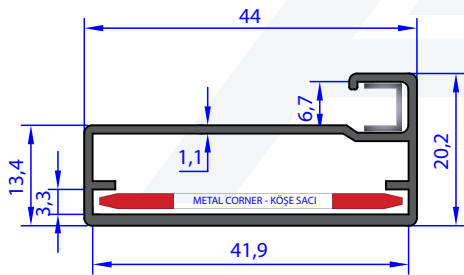
A.3095 WEIGHT 0.438 Kg/m
