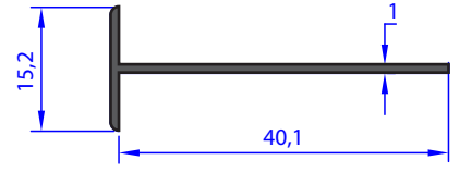
A.4122 WEIGHT 0.149 Kg/m
