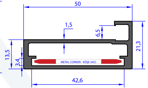
AB 97753 WEIGHT 0.644 Kg/m
