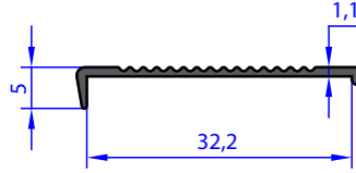
A.4118 WEIGHT 0.102 Kg/m
