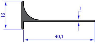
A.4120 WEIGHT 0.202 Kg/m
