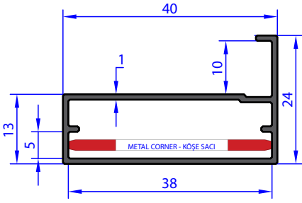
AB 96812 WEIGHT 0.326 Kg/m
