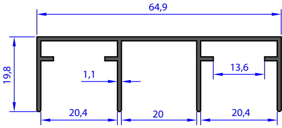
A.3032 WEIGHT 0.441 Kg/m
