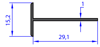
A.4119 WEIGHT 0.132 Kg/m
