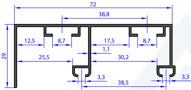
AB 97571 WEIGHT 0.552 Kg/m
