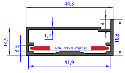
A.3091 WEIGHT 0.445 Kg/m
