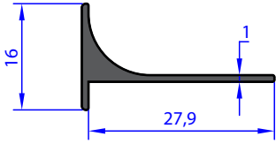
A.4117 WEIGHT 0.172 Kg/m
