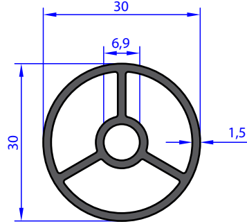
AB 95112 WEIGHT 0.577 Kg/m
