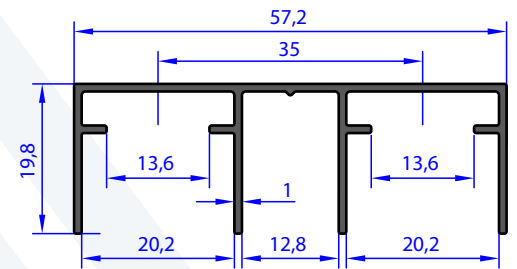
AB 96794 WEIGHT 0.395 Kg/m
