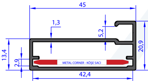
AB 92228 WEIGHT 0.493 Kg/m
