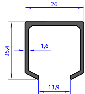
AB 97040 WEIGHT 0.346 Kg/m
