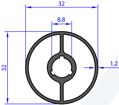
AB 97143 WEIGHT 0.549 Kg/m
