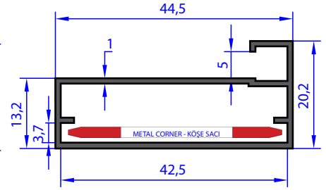
AB 96893 WEIGHT 0.369 Kg/m
