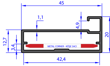
AB 96008 WEIGHT 0.450 Kg/m
