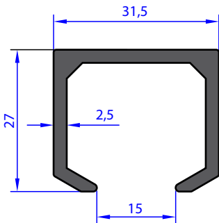
AB 97082 WEIGHT 0.613 Kg/m
