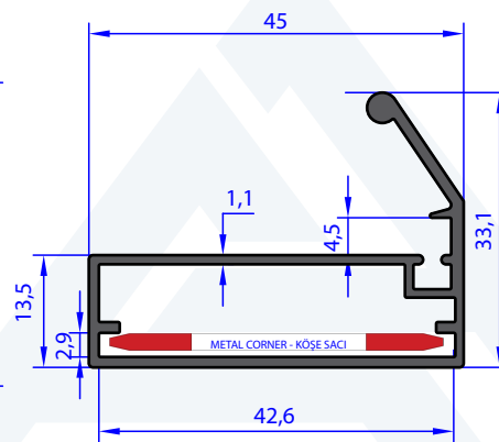
AB 96936 WEIGHT 0.501 Kg/m
