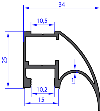
AB 97013 WEIGHT 0.431 Kg/m
