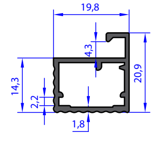
AB 92229 WEIGHT 0.271 Kg/m
