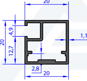
AB 95668 WEIGHT 0.286 Kg/m
