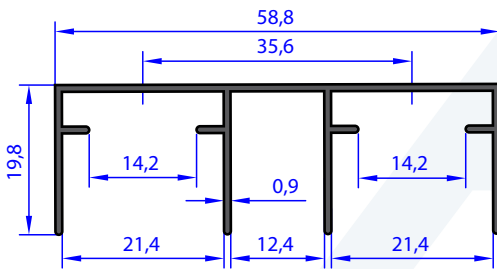
AB 92561 WEIGHT 0.373 Kg/m
