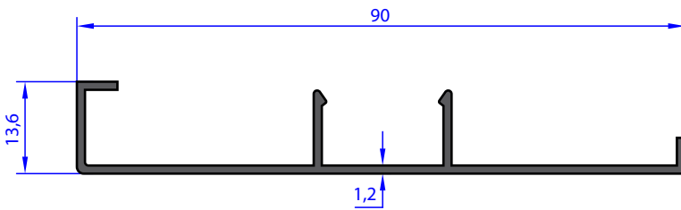
AB 96537 WEIGHT 0.436 Kg/m
