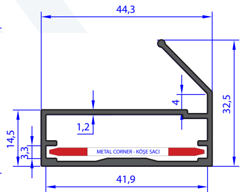
A.4092 WEIGHT 0.509 Kg/m
