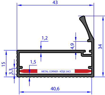
A.3094 WEIGHT 0.490 Kg/m
