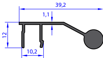
AB 92621 WEIGHT 0.346 Kg/m
