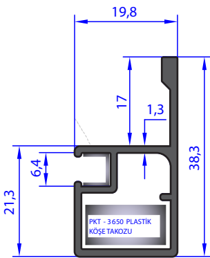
A.3100 WEIGHT 0.405 Kg/m
