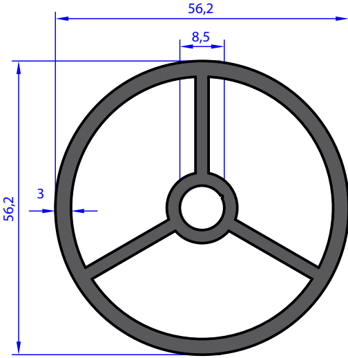
AB 96690 WEIGHT 1.965 Kg/m
