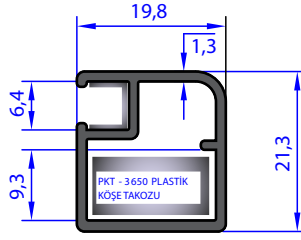
A.3099 WEIGHT 0.281 Kg/m
