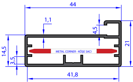
AB 96803 WEIGHT 0.429 Kg/m
