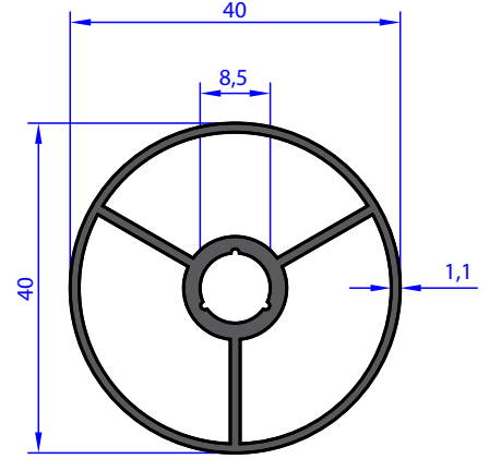
AB 97343 WEIGHT 0.663 Kg/m
