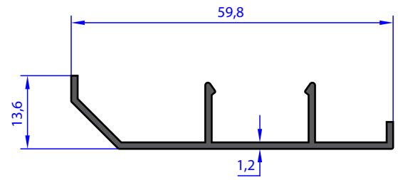
AB 92627 WEIGHT 0.316 Kg/m
