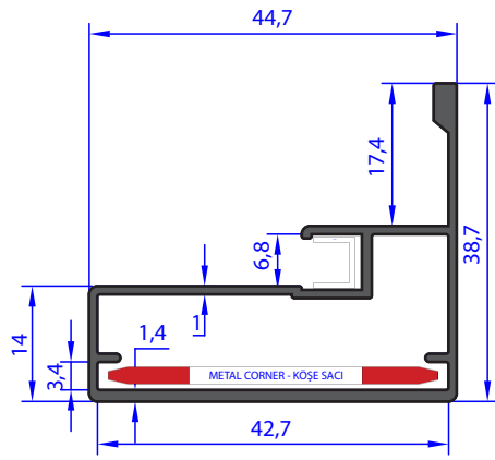
A.3090 WEIGHT 0.538 Kg/m
