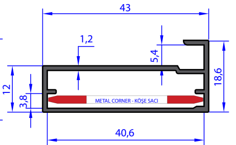
AB 92237 WEIGHT 0.383 Kg/m
