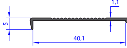
A.4121 WEIGHT 0.121 Kg/m
