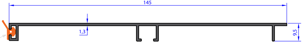
BFTL - 3840 BAZA FİTİLİ - (BASE GASKET)
