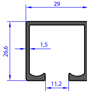
AB 97537 WEIGHT 0.418 Kg/m
