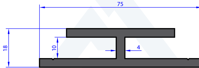
AB 92595 WEIGHT 1.462 Kg/m
